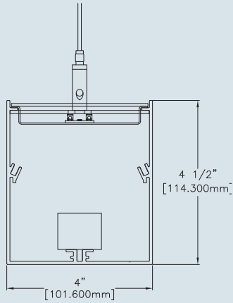
Clear Acrylic (CA) lens shown. See page 4 for other lens details.
