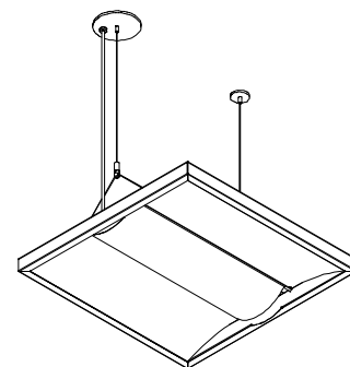
ACY Suspended Aircraft Cable (1/16" dia., 48"L)
